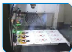
Auto job changeover The sensor detects each QRcode which contains cutting information to change the job automatically, in real time!
